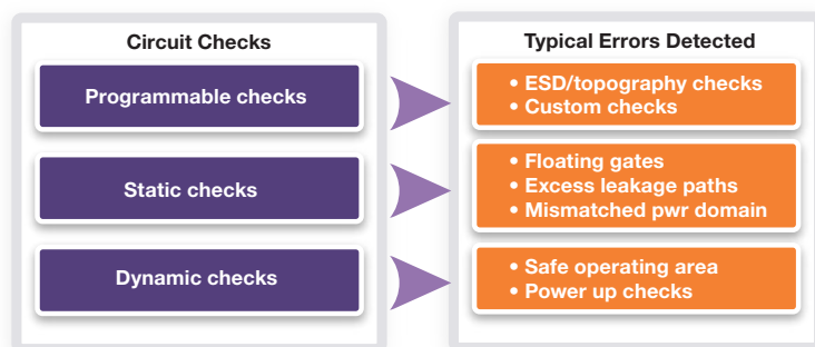
Figure 1: CustomSim native circuit checks enable ERC & low power verification
